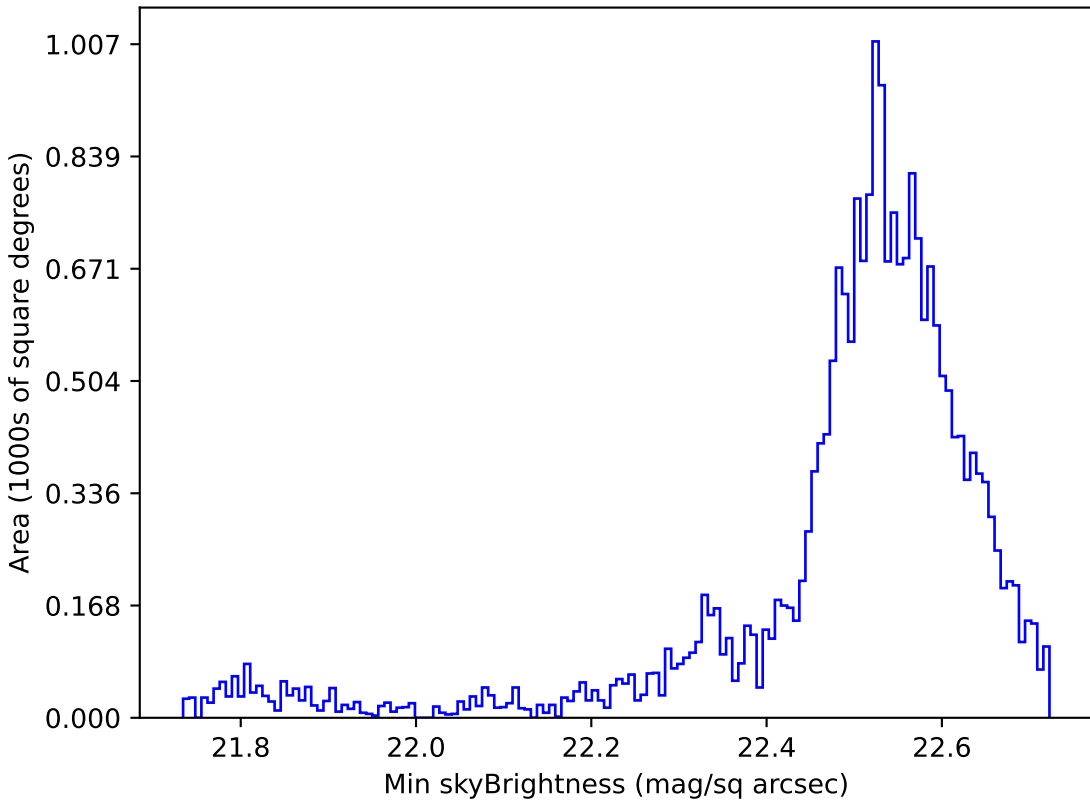
too_ignore_5_1v3.4_10yrs Yr 1 u band: Min skyBrightness
