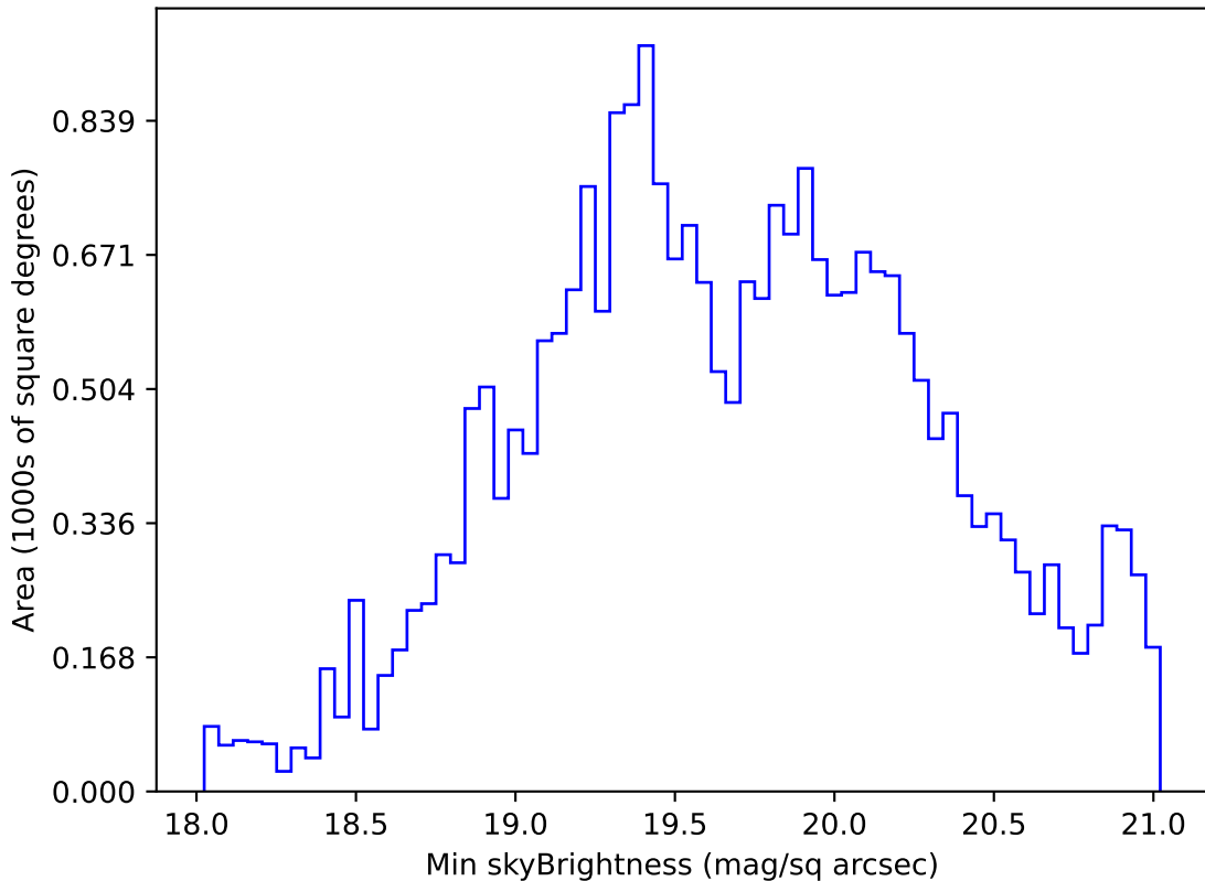
too_ignore_5_1v3.4_10yrs Yr 1 r band: Min skyBrightness
