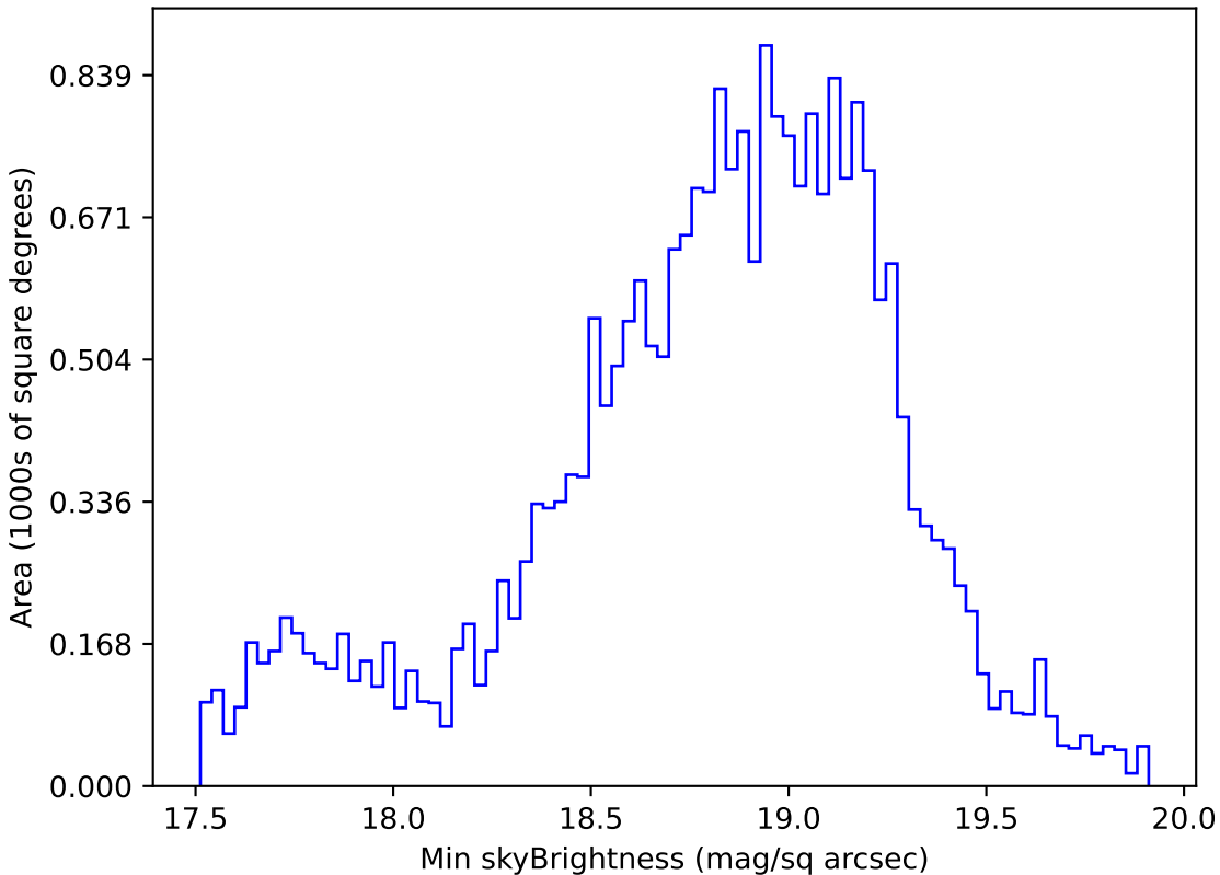
too_ignore_5_1v3.4_10yrs Yr 1 i band: Min skyBrightness
