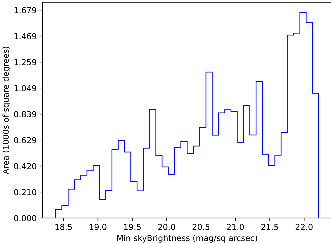
too_ignore_5_1v3.4_10yrs Yr 1 g band: Min skyBrightness
