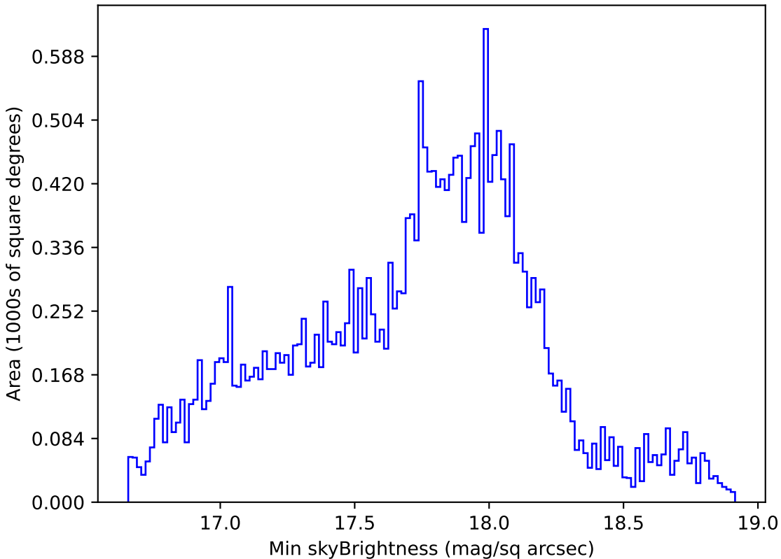
too_ignore_5_1v3.4_10yrs Yr 1 all bands: Min skyBrightness
