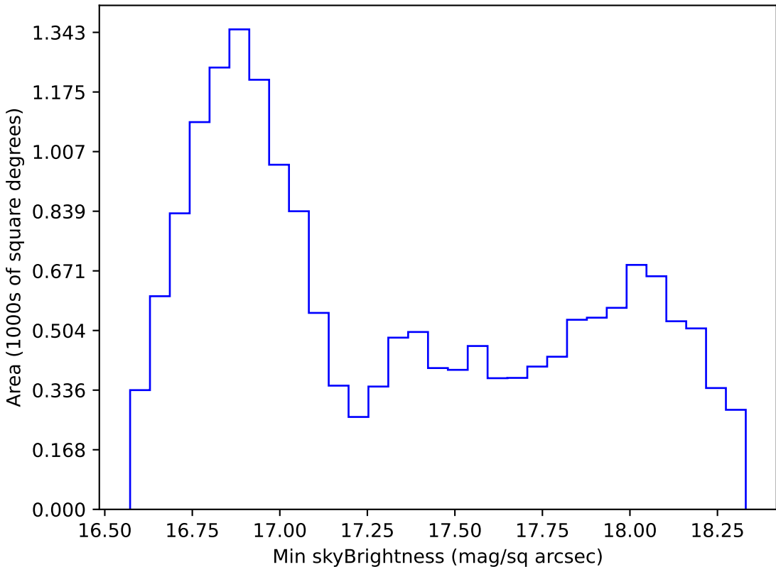
too_ignore_5_1v3.4_10yrs WFD z band: Min skyBrightness
