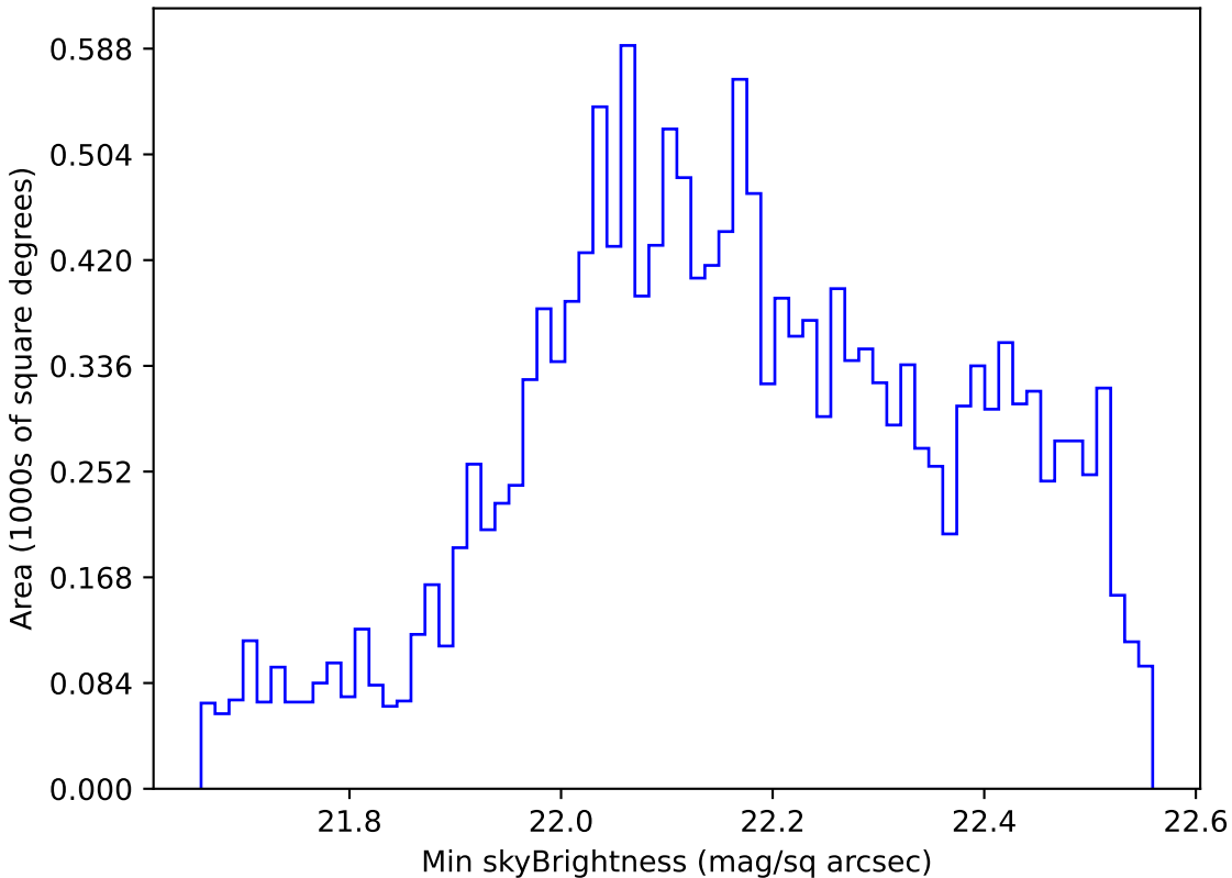
too_ignore_5_1v3.4_10yrs WFD u band: Min skyBrightness
