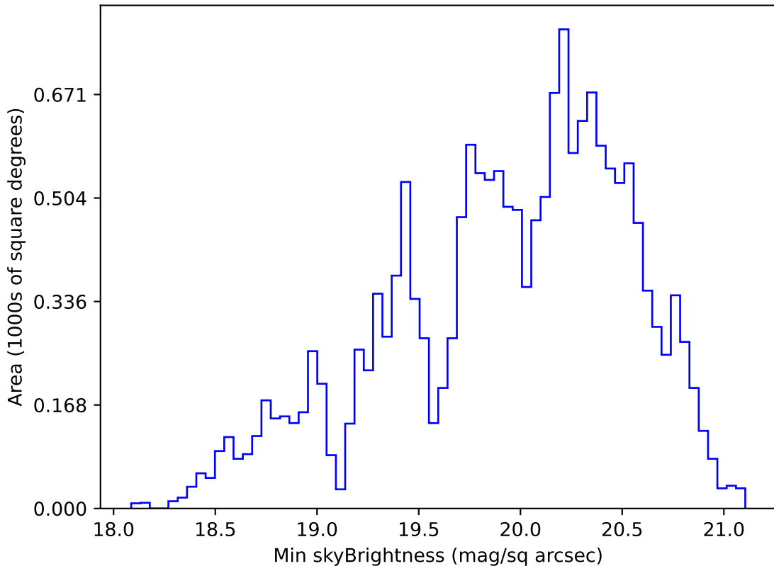
too_ignore_5_1v3.4_10yrs WFD g band: Min skyBrightness
