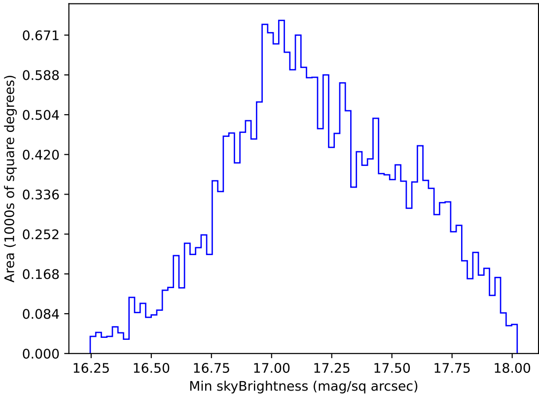
too_ignore_5_1v3.4_10yrs All sky y band: Min skyBrightness
