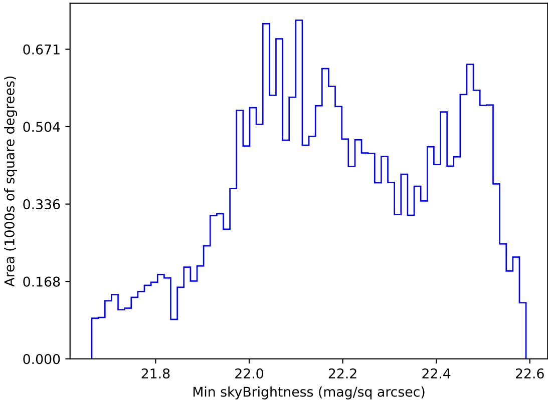
too_ignore_5_1v3.4_10yrs All sky u band: Min skyBrightness
