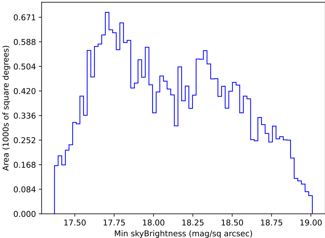
too_ignore_5_1v3.4_10yrs All sky i band: Min skyBrightness
