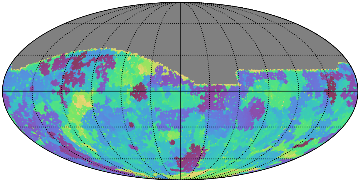
too_ignore_5_1v3.4_10yrs All sky g band: Min skyBrightness
