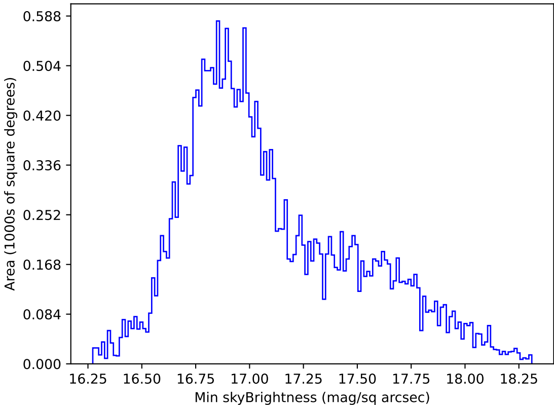
too_ignore_5_1v3.4_10yrs All sky all bands: Min skyBrightness
