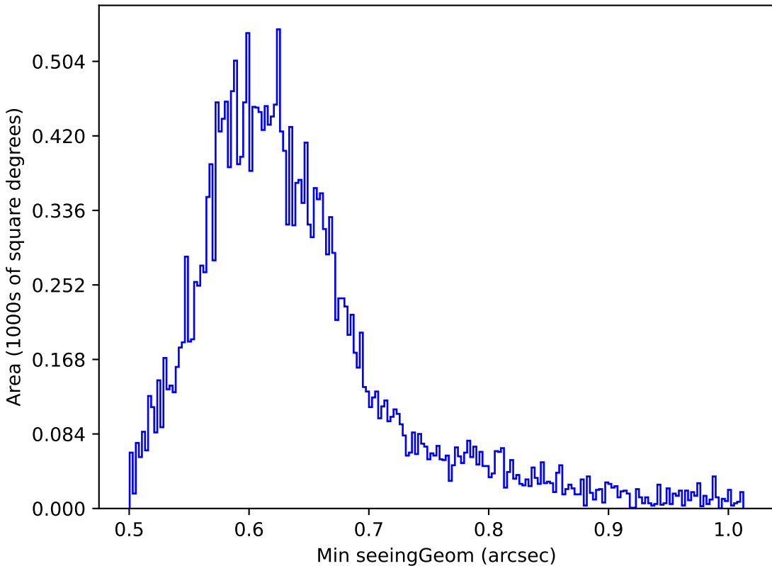
too_ignore_5_1v3.4_10yrs Yr 1 z band: Min seeingGeom
