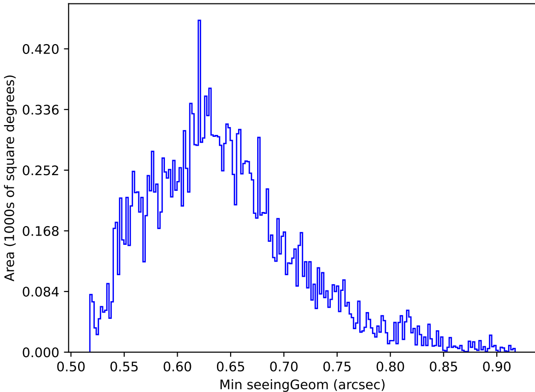
too_ignore_5_1v3.4_10yrs Yr 1 y band: Min seeingGeom
