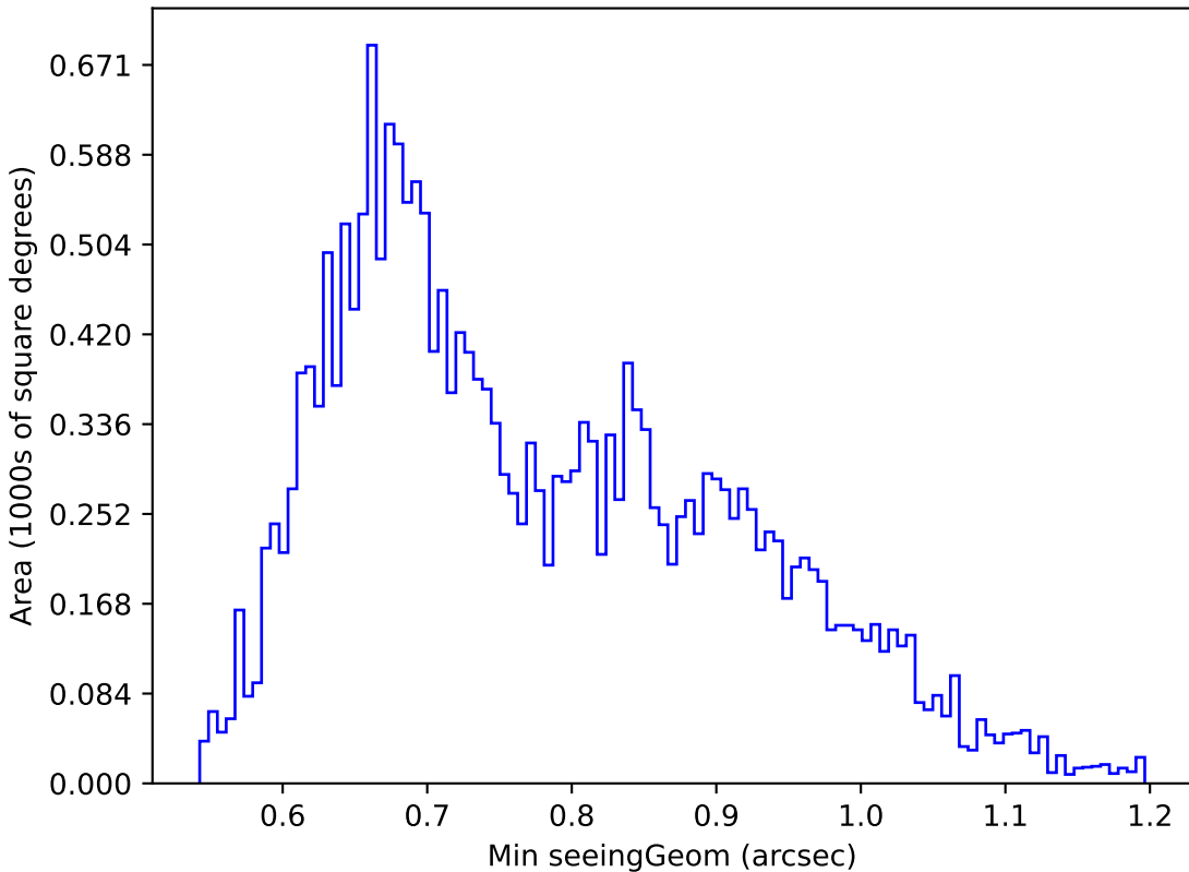
too_ignore_5_1v3.4_10yrs Yr 1 u band: Min seeingGeom
