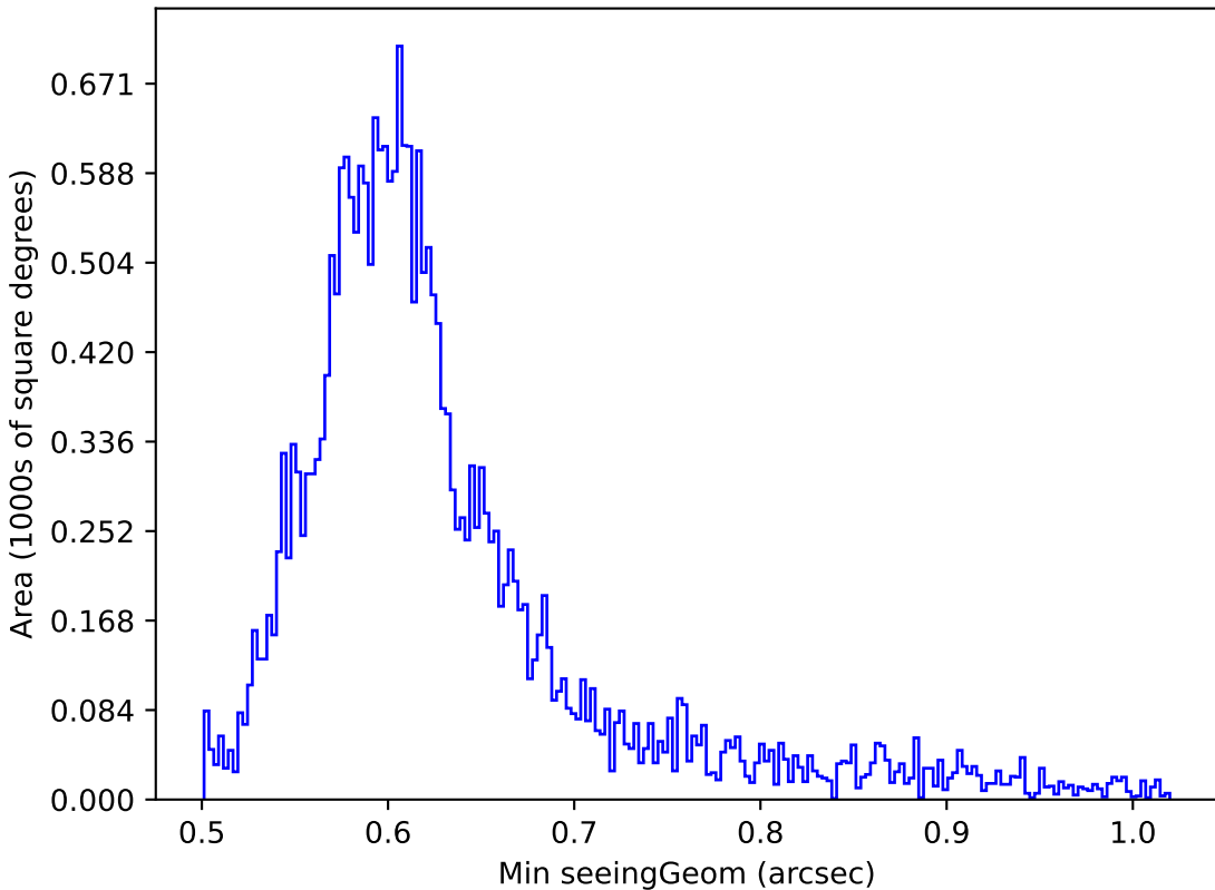
too_ignore_5_1v3.4_10yrs Yr 1 i band: Min seeingGeom
