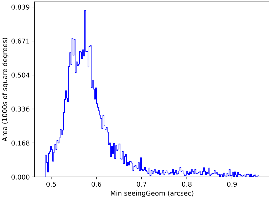
too_ignore_5_1v3.4_10yrs Yr 1 all bands: Min seeingGeom
