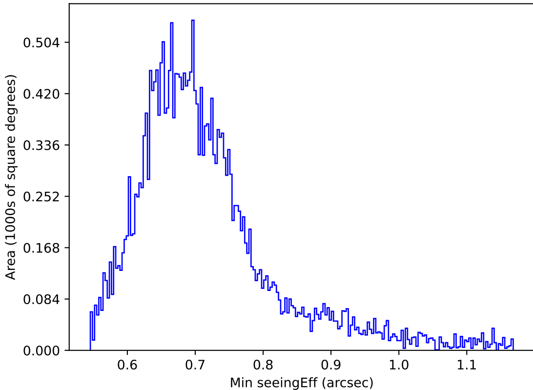
too_ignore_5_1v3.4_10yrs Yr 1 z band: Min seeingEff
