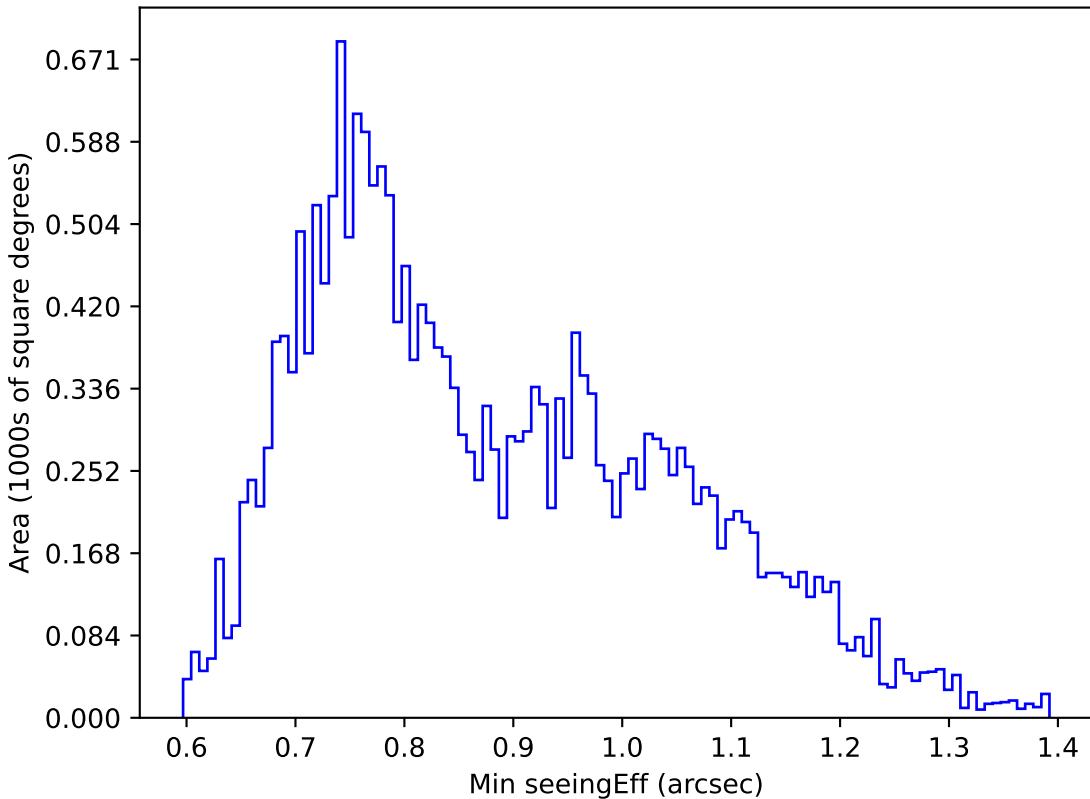
too_ignore_5_1v3.4_10yrs Yr 1 u band: Min seeingEff
