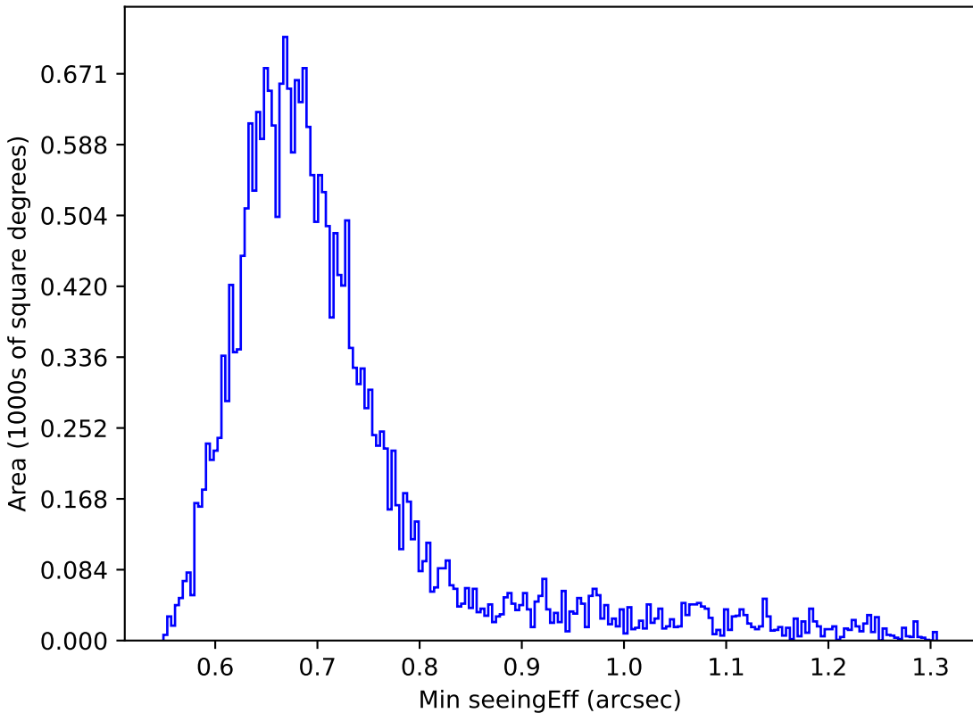
too_ignore_5_1v3.4_10yrs Yr 1 r band: Min seeingEff
