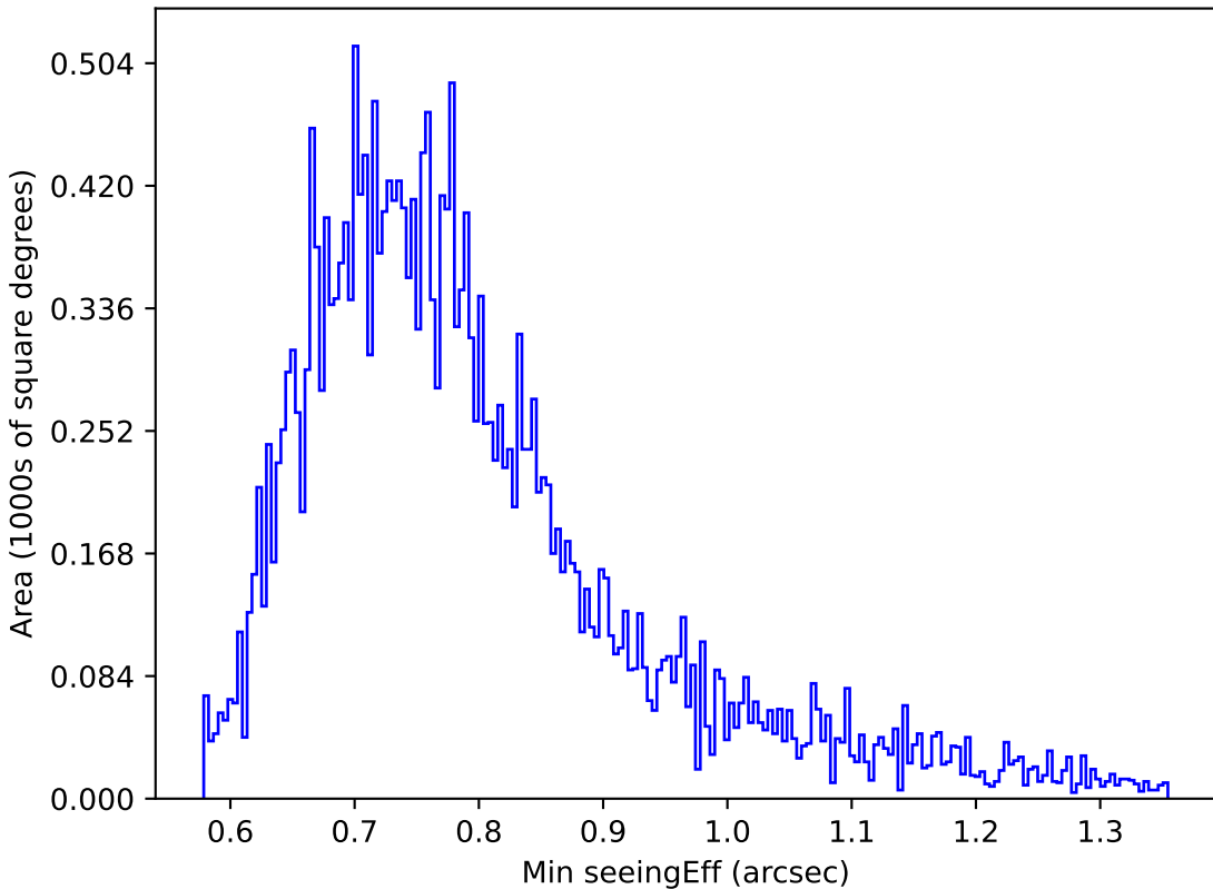
too_ignore_5_1v3.4_10yrs Yr 1 g band: Min seeingEff
