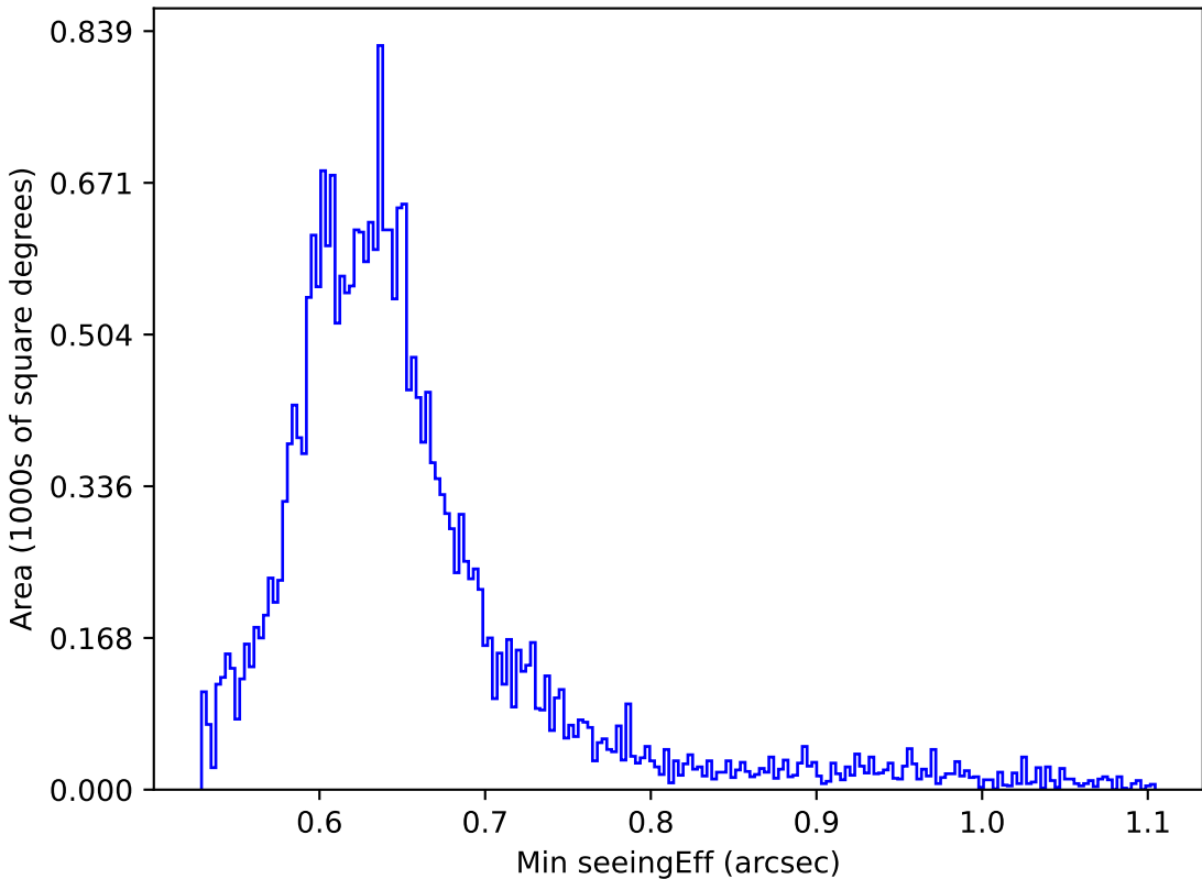
too_ignore_5_1v3.4_10yrs Yr 1 all bands: Min seeingEff
