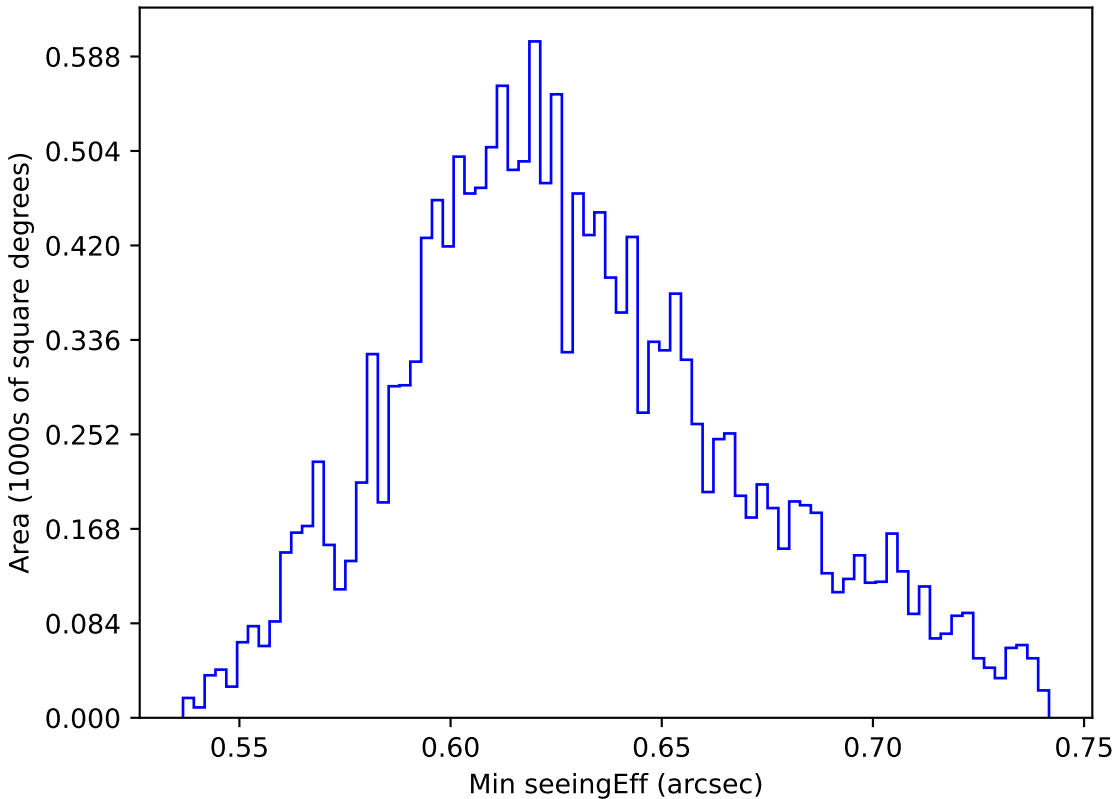
too_ignore_5_1v3.4_10yrs WFD y band: Min seeingEff
