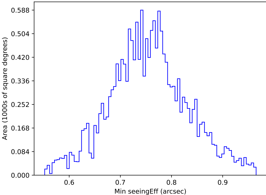
too_ignore_5_1v3.4_10yrs WFD u band: Min seeingEff
