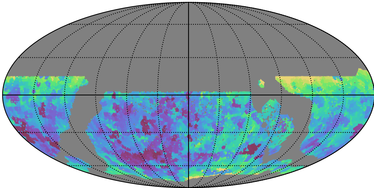
too_ignore_5_1v3.4_10yrs WFD r band: Min seeingEff
