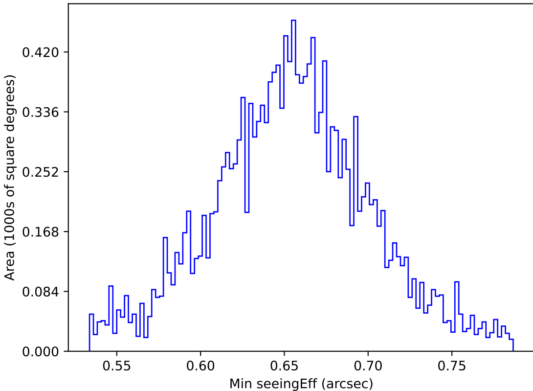
too_ignore_5_1v3.4_10yrs WFD g band: Min seeingEff
