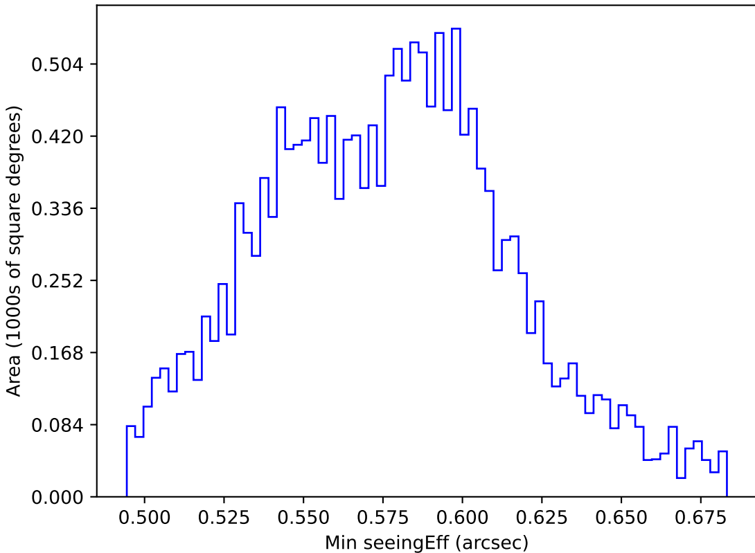
too_ignore_5_1v3.4_10yrs WFD all bands: Min seeingEff
