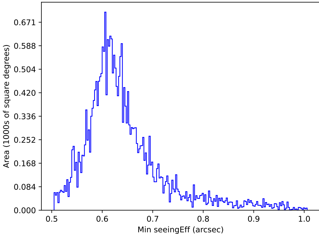
too_ignore_5_1v3.4_10yrs All sky z band: Min seeingEff
