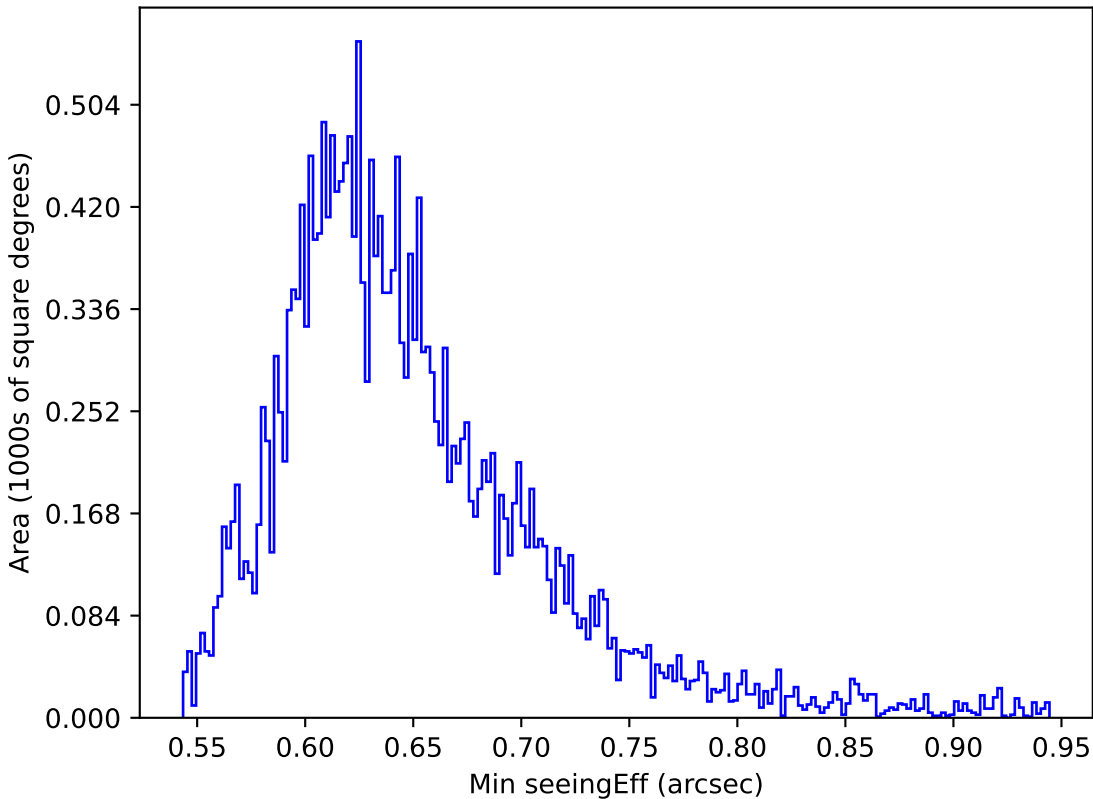
too_ignore_5_1v3.4_10yrs All sky y band: Min seeingEff
