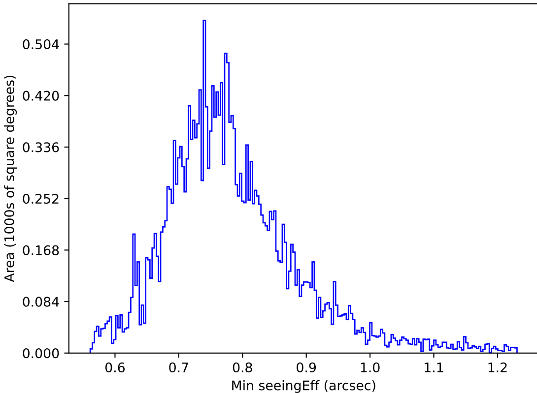
too_ignore_5_1v3.4_10yrs All sky u band: Min seeingEff
