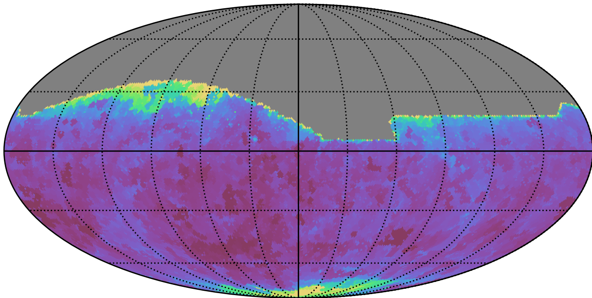
too_ignore_5_1v3.4_10yrs All sky r band: Min seeingEff
