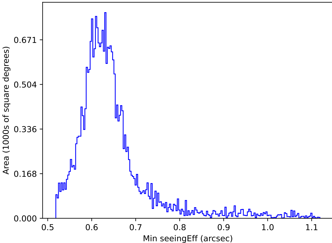
too_ignore_5_1v3.4_10yrs All sky r band: Min seeingEff
