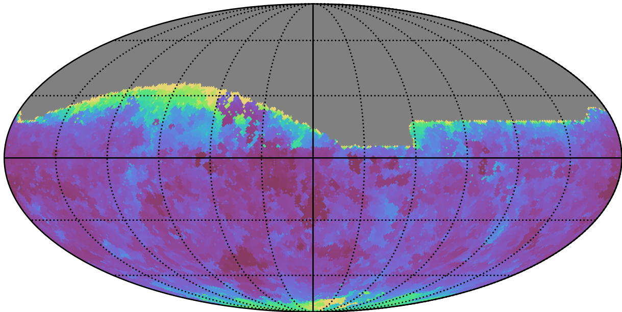
too_ignore_5_1v3.4_10yrs All sky g band: Min seeingEff
