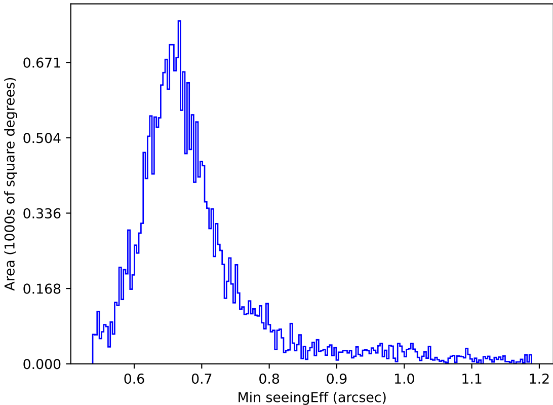
too_ignore_5_1v3.4_10yrs All sky g band: Min seeingEff
