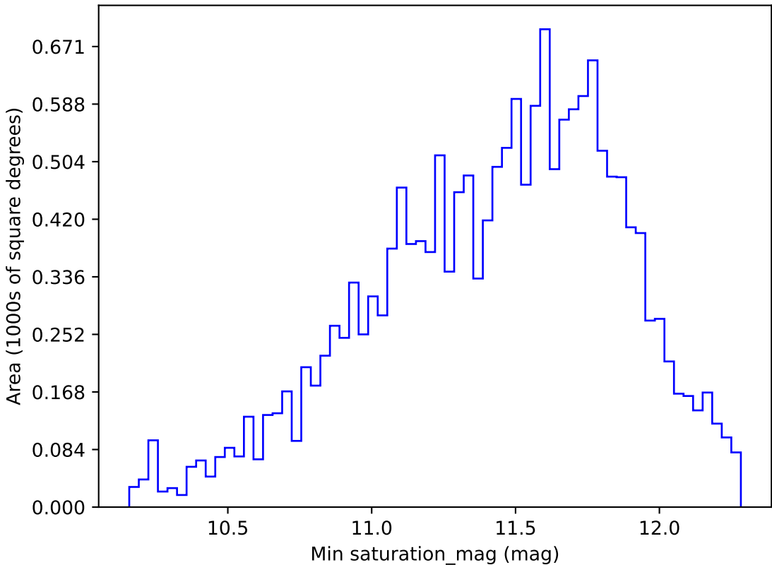
too_ignore_5_1v3.4_10yrs WFD u band: Min saturation_mag
