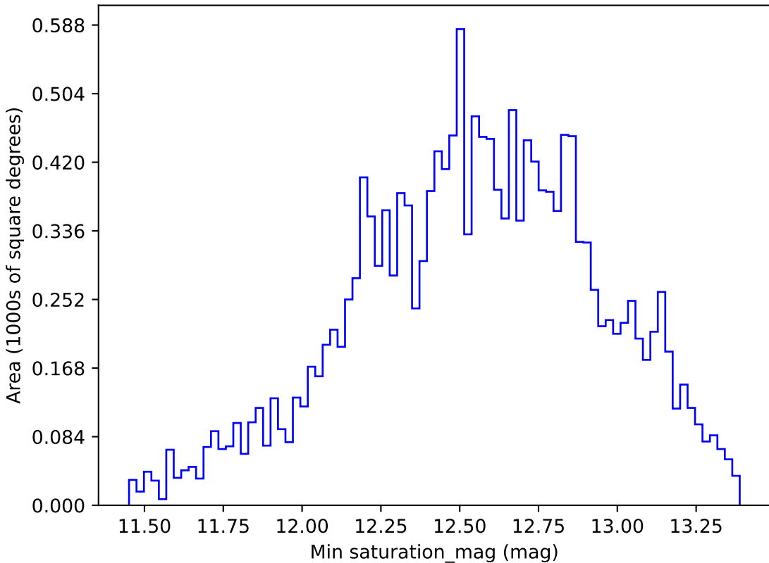
too_ignore_5_1v3.4_10yrs WFD r band: Min saturation_mag
