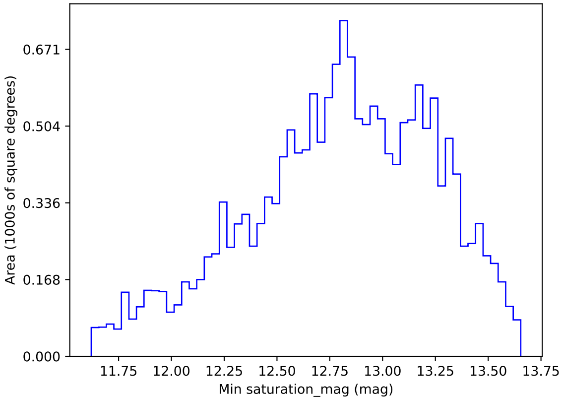
too_ignore_5_1v3.4_10yrs WFD g band: Min saturation_mag
