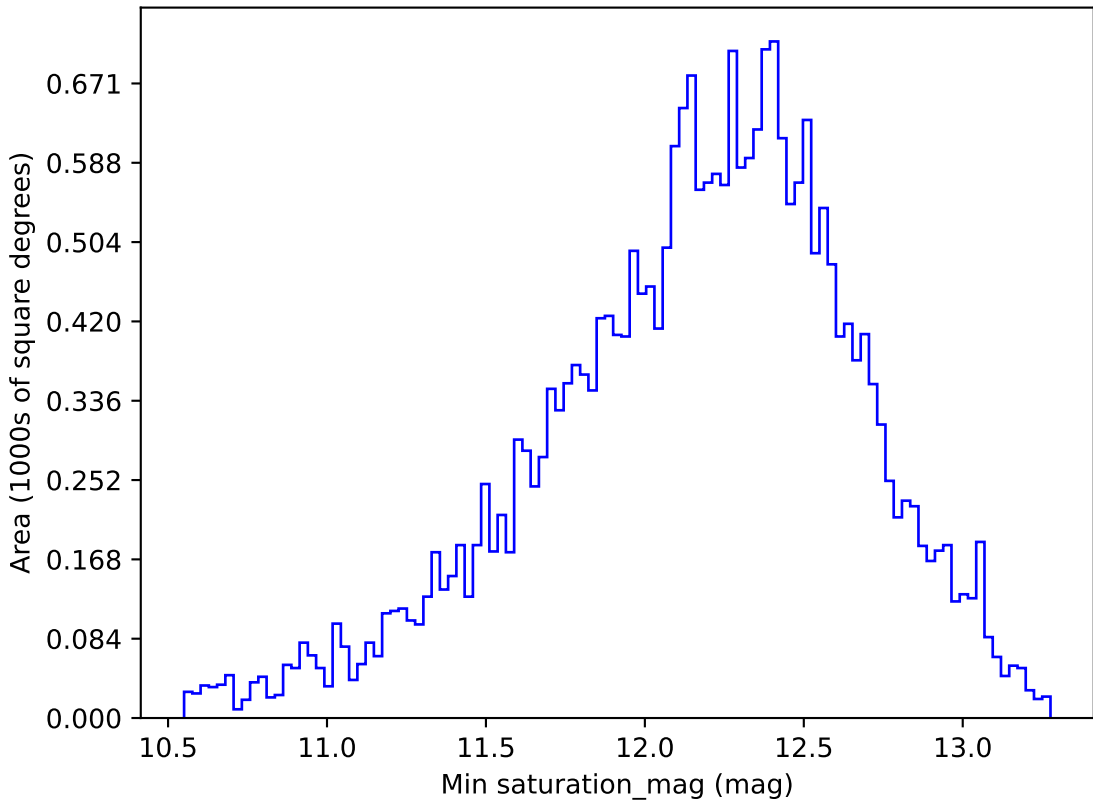
too_ignore_5_1v3.4_10yrs All sky z band: Min saturation_mag
