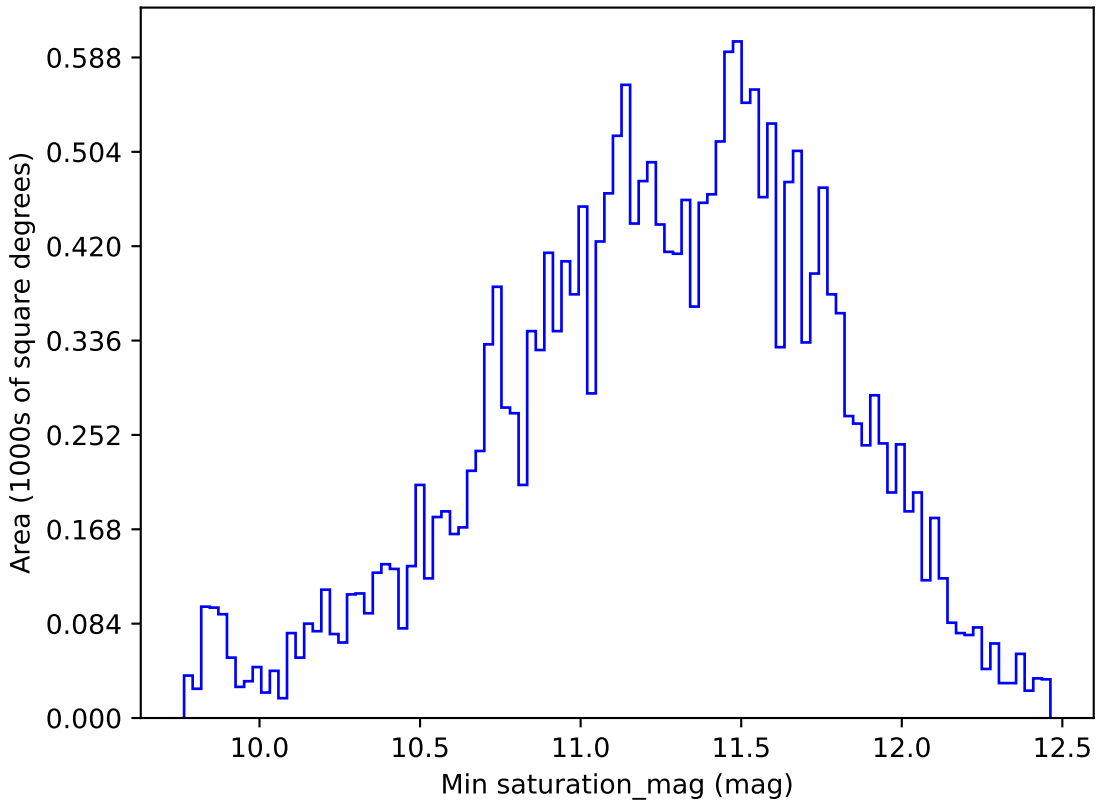
too_ignore_5_1v3.4_10yrs All sky y band: Min saturation_mag
