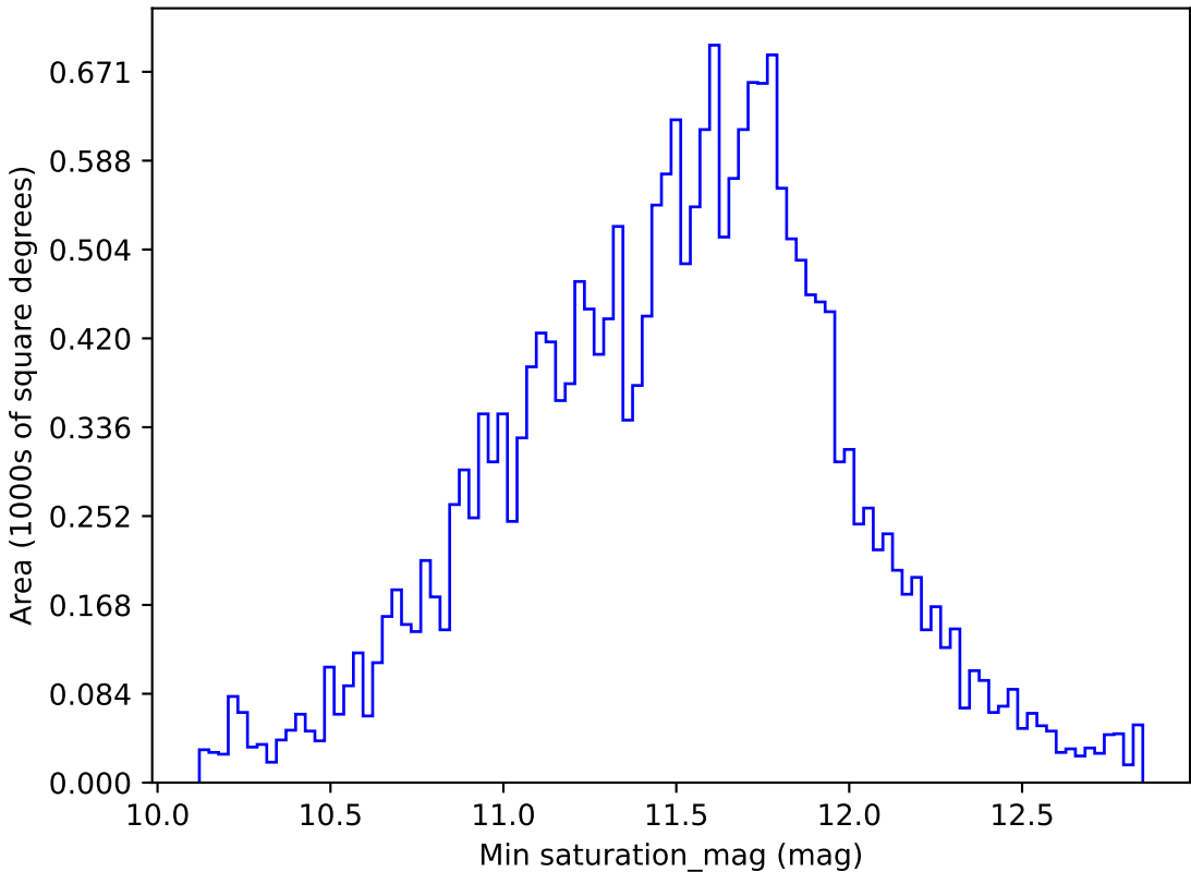
too_ignore_5_1v3.4_10yrs All sky u band: Min saturation_mag
