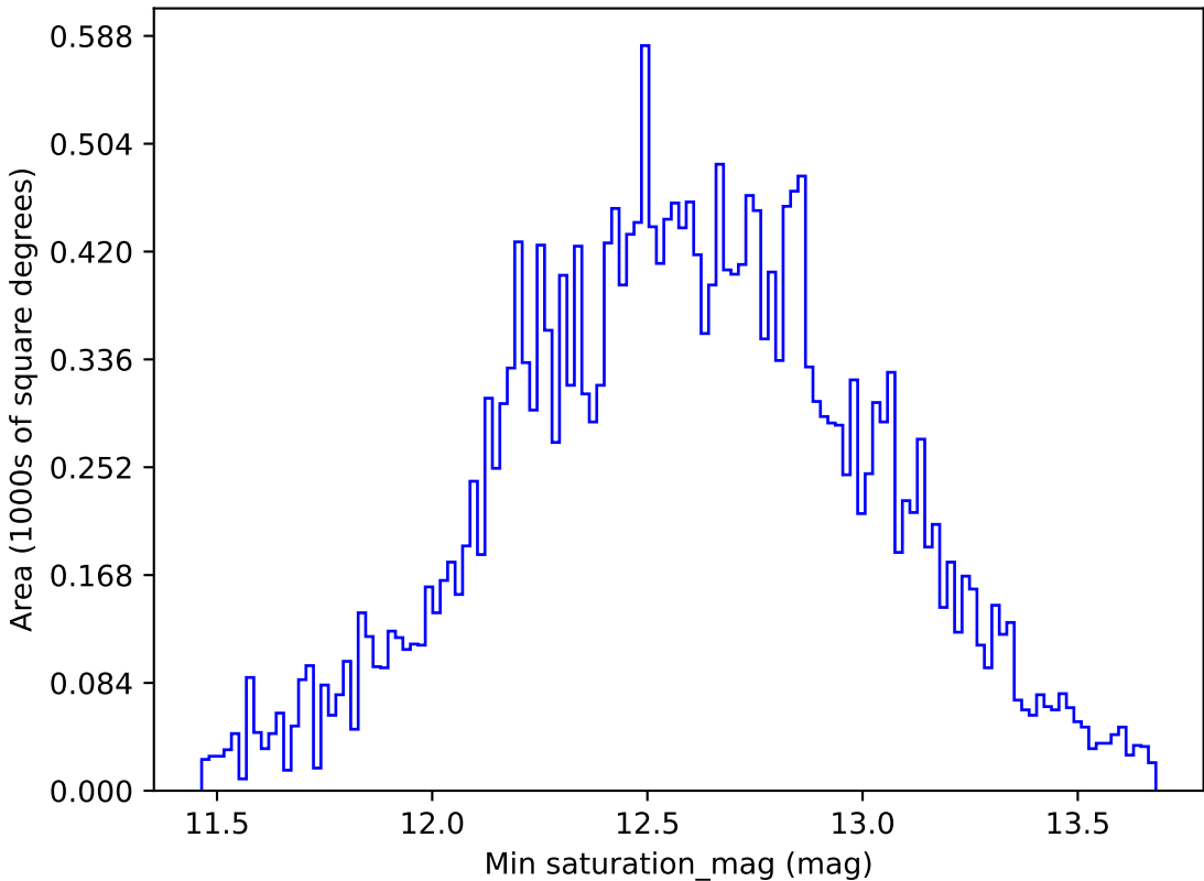
too_ignore_5_1v3.4_10yrs All sky r band: Min saturation_mag
