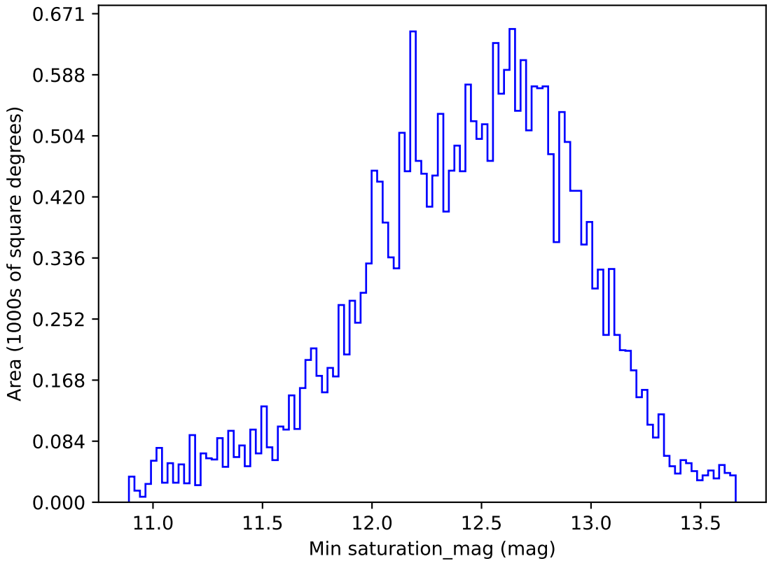
too_ignore_5_1v3.4_10yrs All sky i band: Min saturation_mag
