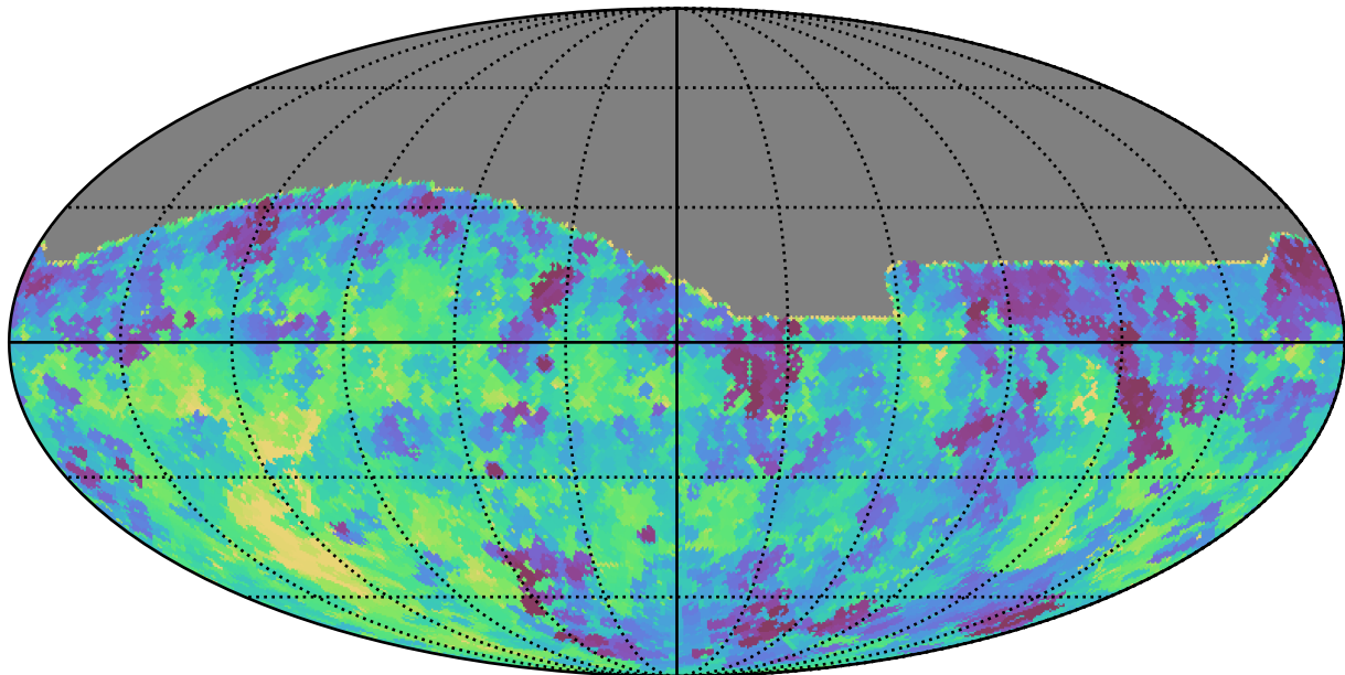
too_ignore_5_1v3.4_10yrs All sky g band: Min saturation_mag
