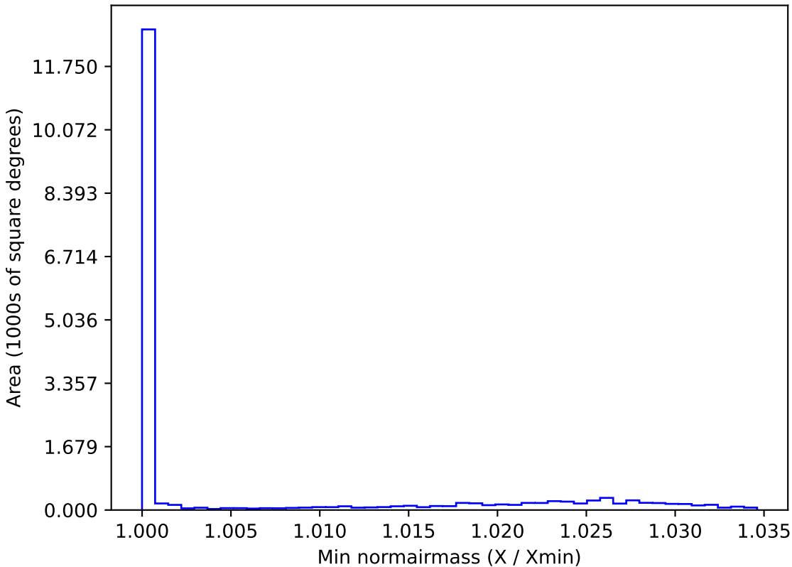
too_ignore_5_1v3.4_10yrs WFD i band: Min normairmass
