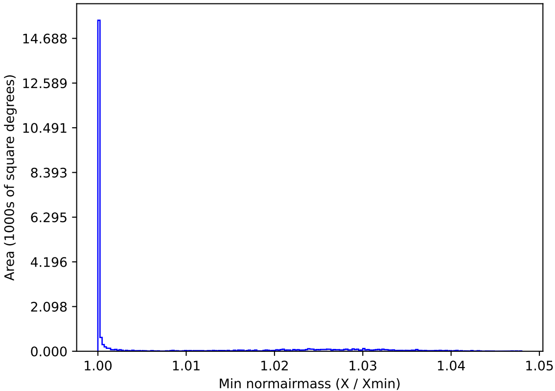
too_ignore_5_1v3.4_10yrs All sky y band: Min normairmass
