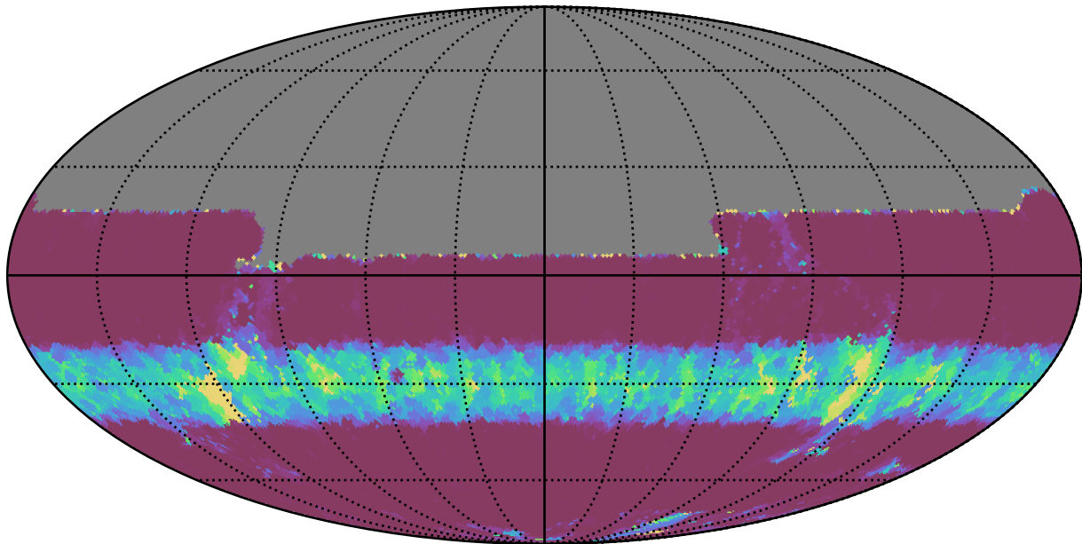
too_ignore_5_1v3.4_10yrs All sky u band: Min normairmass
