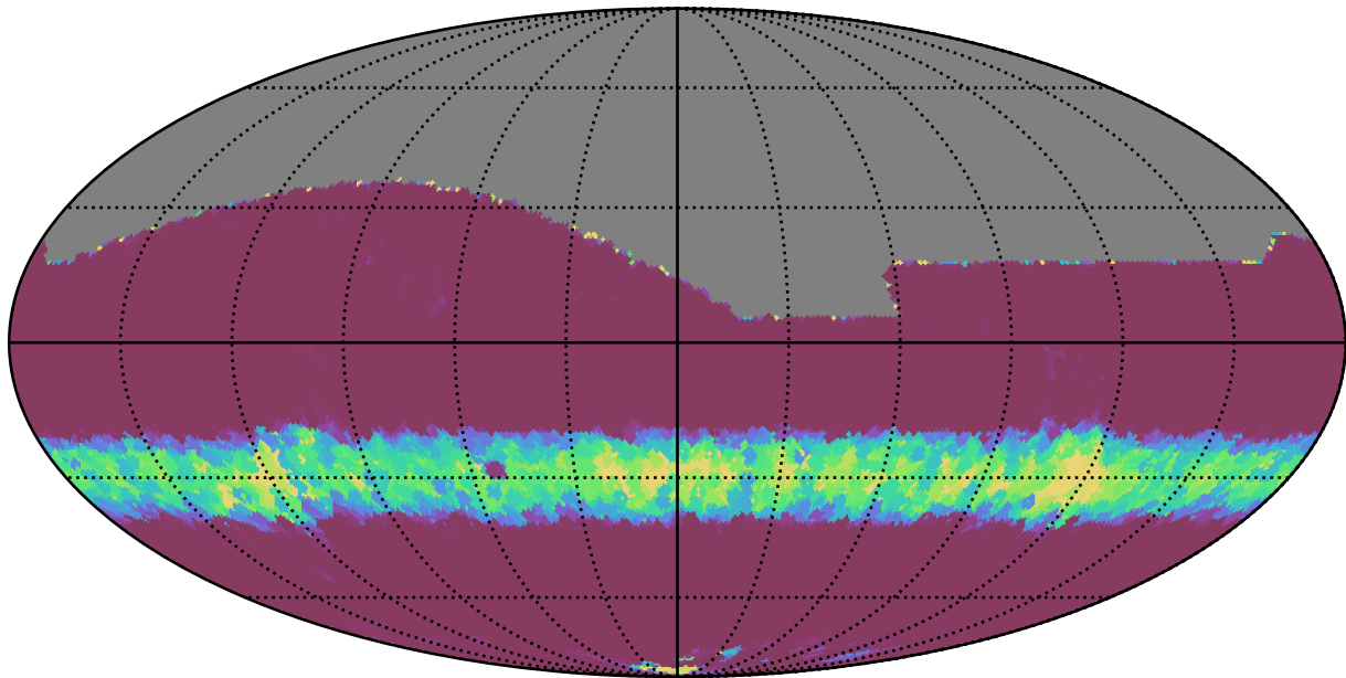
too_ignore_5_1v3.4_10yrs All sky r band: Min normairmass
