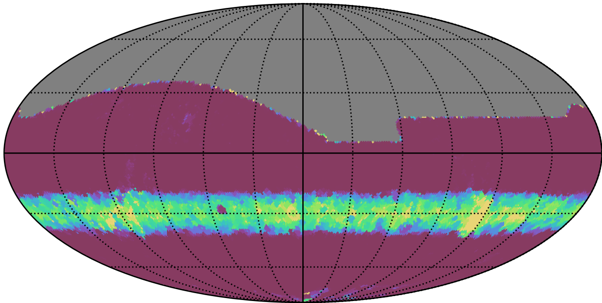
too_ignore_5_1v3.4_10yrs All sky i band: Min normairmass
