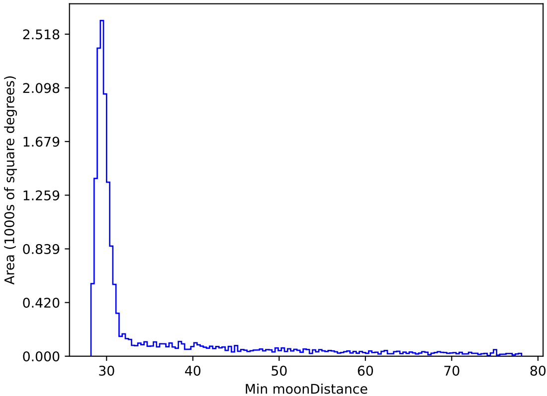
too_ignore_5_1v3.4_10yrs WFD y band: Min moonDistance
